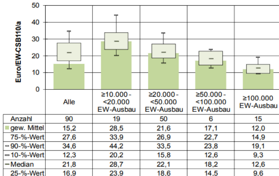
Figure 7: Costs for wastewater treatment in UWWTPs with P_{tot} -removal according to the size of the UWWTP (Lindtner and Vohryzka, 2013)
