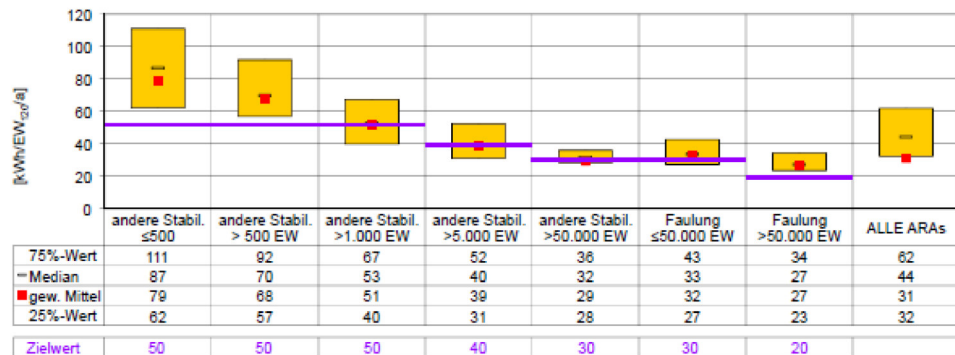
Figure 14: Specific energy consumption [kWh/PE/a] per size class and type of sludge stabilization and potential for energy savings (ÖWAV-KAN survey 2019 in ÖWAV, 2020c)
