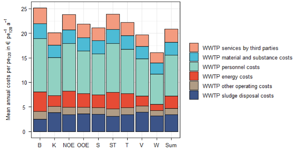
Figure 22: Operating costs for wastewater treatment in Austria and in different provinces (Amann et al., 2021 based on Assmann et al., 2020 and Lindtner, 2018)
