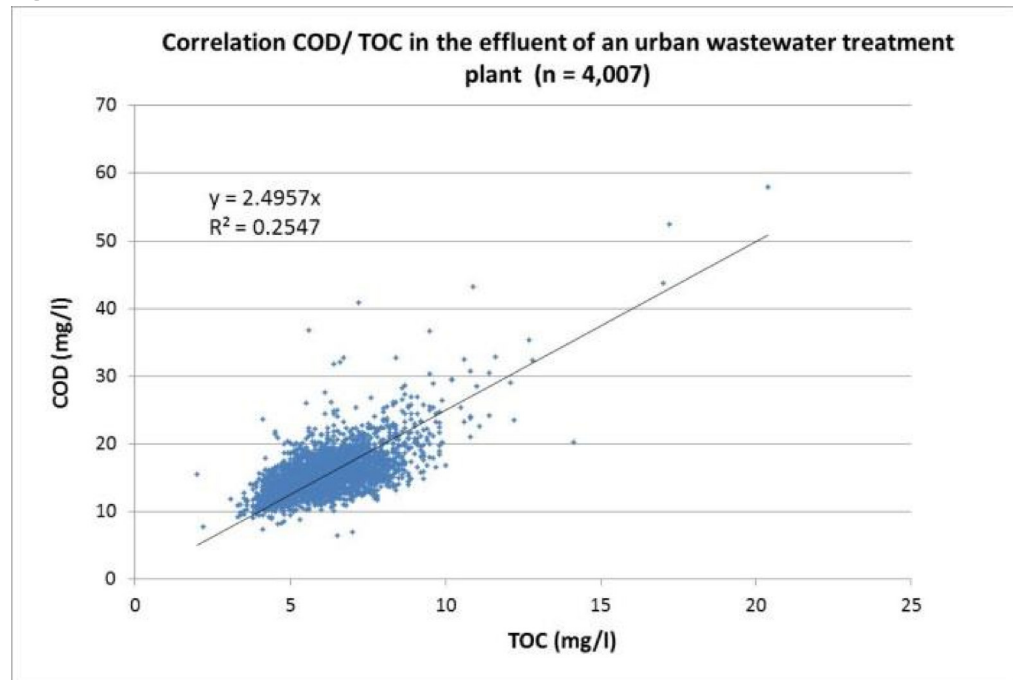
Figure 26: Correlation COD/TOC in UWWTP \geq 100\,000 PE
