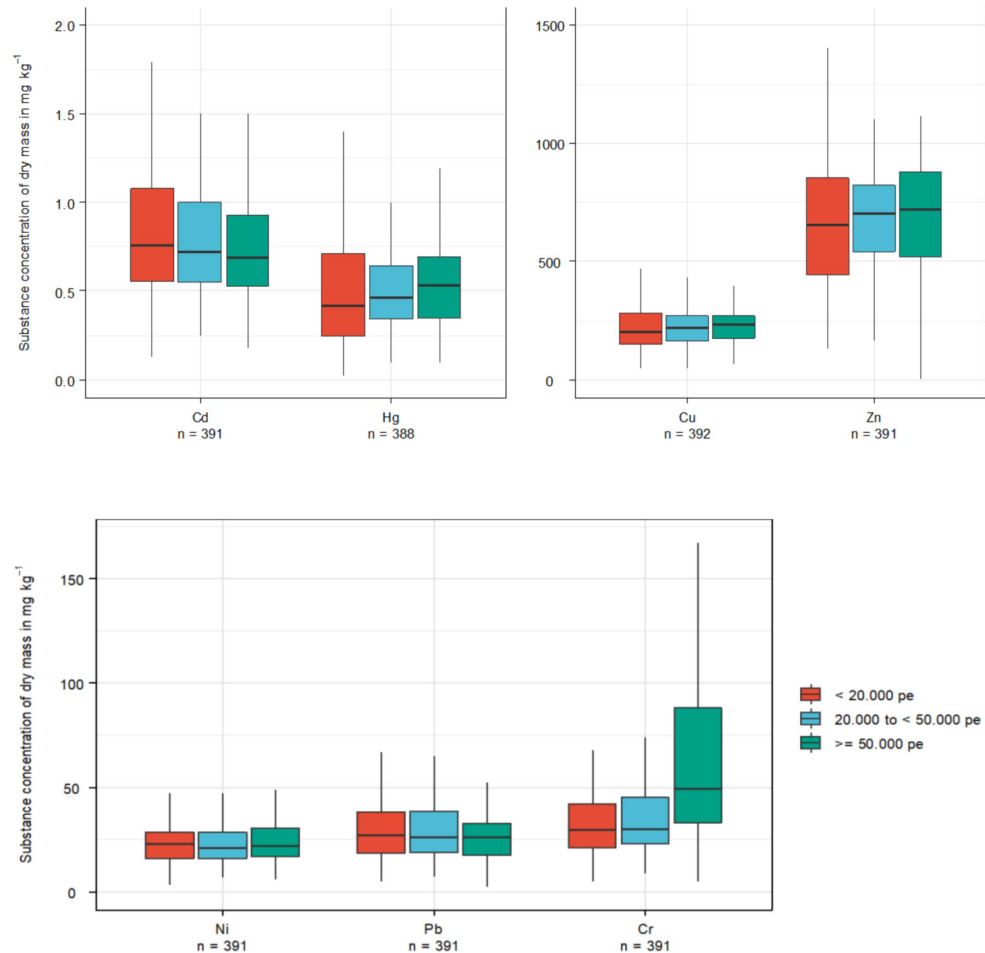
Figure 20: Heavy metal concentrations in municipal sewage sludges from UWWTPs of different size categories in Austria, 2006 – 2020. Data from 130 UWWTPs < 20,000 PE, 72 UWWTPs 20,000 PE -50,000 PE and 43 UWWTPs > 50,000 PE (Amann, 2021 based on sludge certificates)
