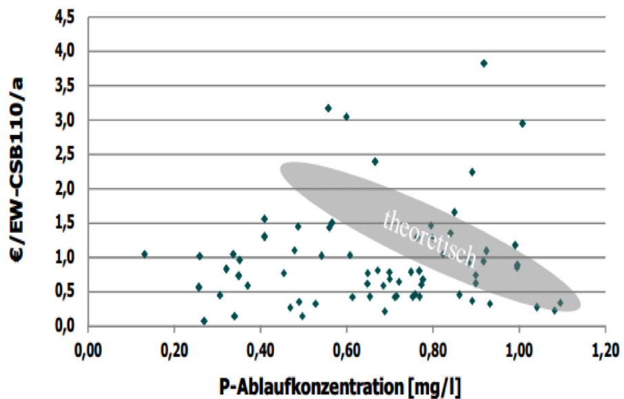
Figure 9: Costs for precipitants versus P_{\text{tot}} concentrations in the effluent (Lindtner and Vohryzka, 2013)
