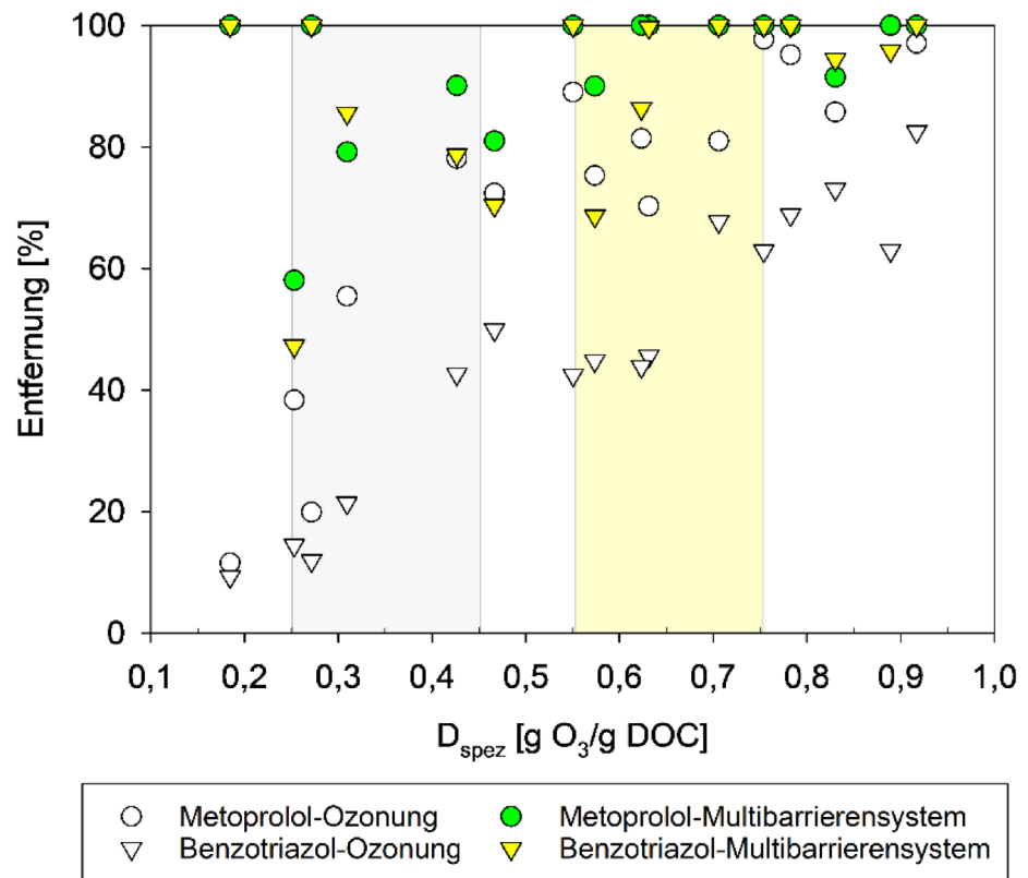
Figure 10: Metoprolol and benzotriazole abatement in ozonation and in a multibarrier-system combining ozonation and granular activated carbon (Krampe et al., 2020)
