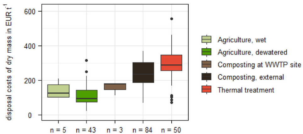
Figure 21: Costs of different sludge reuse and disposal routes (2015-2018, adopted from Damm et al. 2020)
