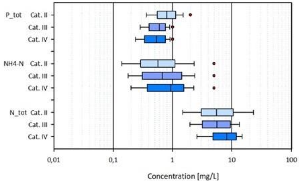
Figure 6: Median effluent concentrations of P_{tot} , NH_4-N and N_{tot} per size class (reference years 2010 –2019) and emission limit value (red dots) according to the 1 st AEVKA (box-plot showing the median, the 25% and 75%-percentile as borders of the box and the 10% and 90% percentile as whiskers)
