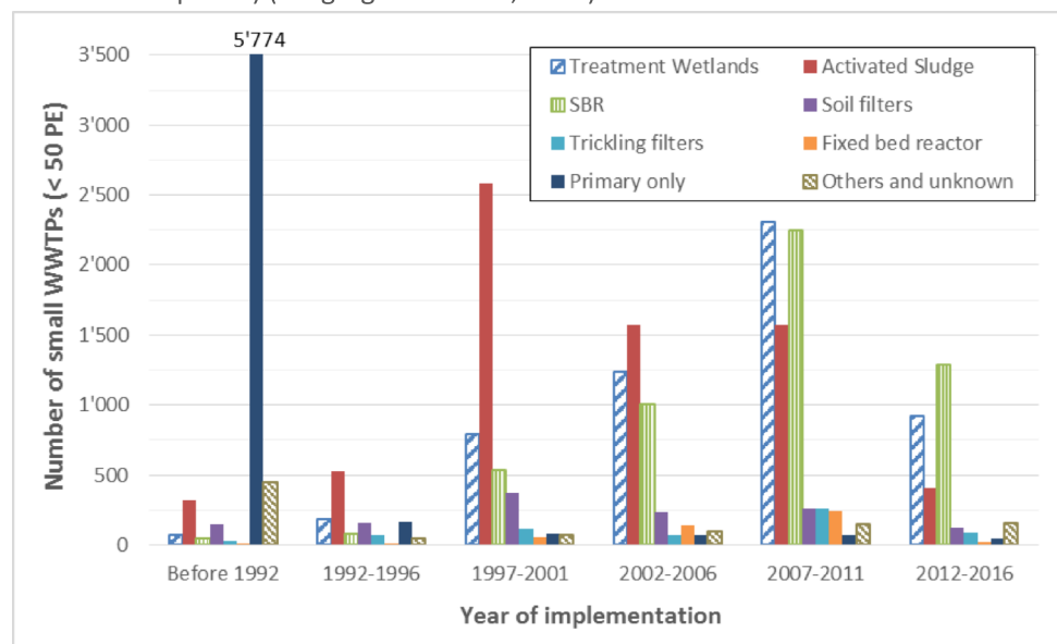
Figure 4: Year of commissioning of different treatment technologies applied for small WWTPs ≤ 50 PE in AT (the category "Unknown and others" includes 52 MBR and 131 RBC plants) (Langergraber et al., 2018)
