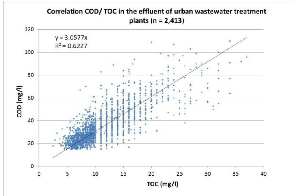
Figure 23: Correlation COD/TOC in UWWTP
