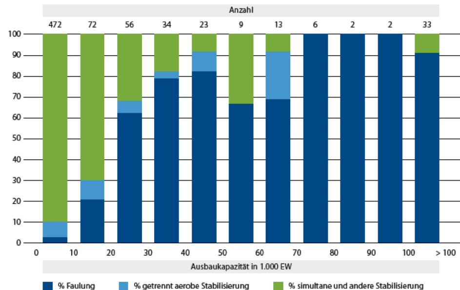
Figure 13: Percentage of UWWTPs with aerobic and anaerobic sludge stabilization (ÖWAV, 2019)
