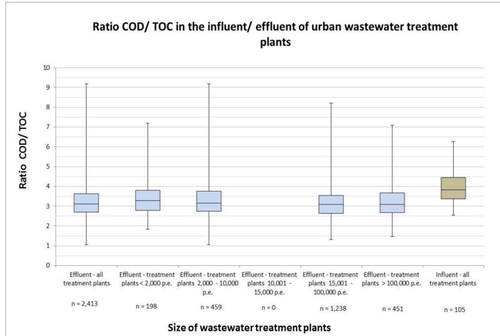
Figure 25: Ratio COD/TOC in UWWTP per size category (the box shows the median value and the 25 & 75% quartiles)
