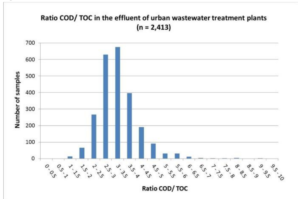
Figure 24: Ratio COD/TOC in UWWTP
