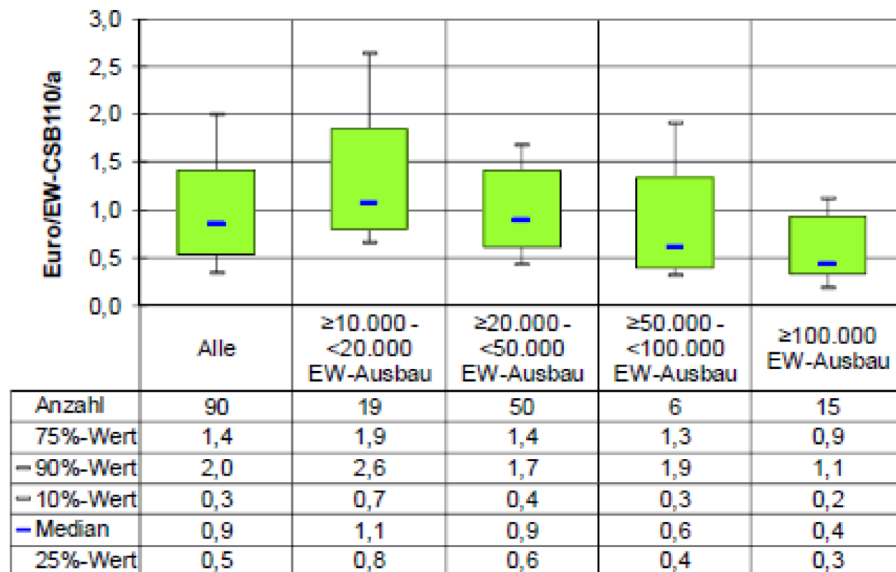
Figure 8: Specific costs for precipitants according to the size of the UWWTP (Lindtner and Vohryzka, 2013)
