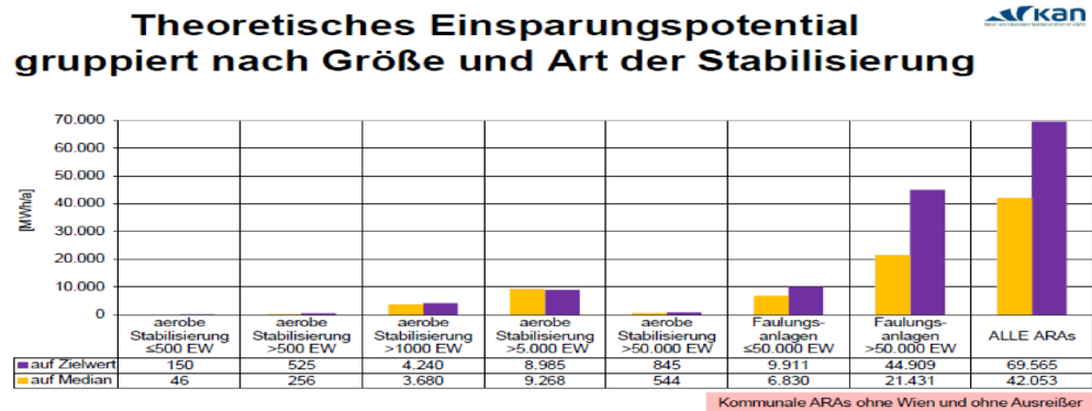
Figure 15: Potential energy savings grouped according to size classes and type of sludge stabilization (Lindtner 2019 in ÖWAV, 2020c)
