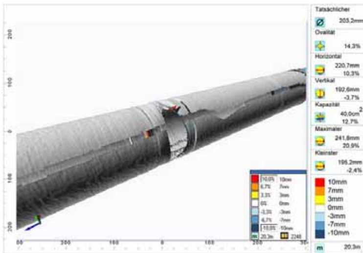
Abbildung 16 - Laser Profiler 3D-Modell (Hartl, 2009)
